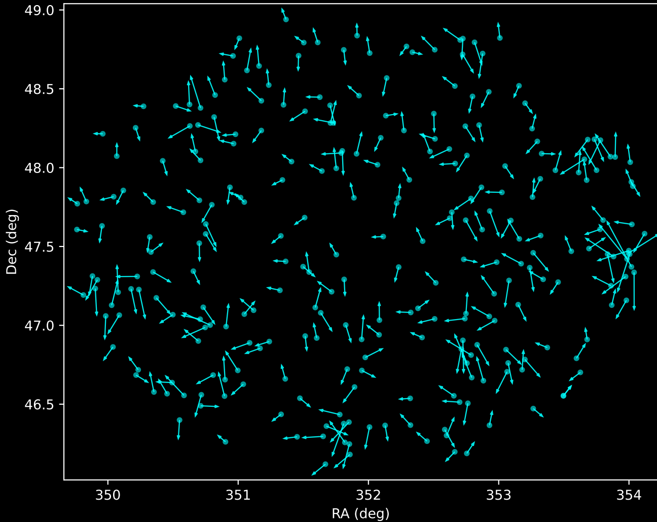
APOGEE DR17 Noise Stream Proper Motion Vectors (n=272)
