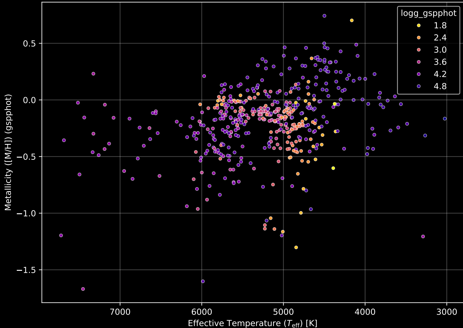
APOGEE DR17 Field: [N6229] Stellar Population Parameters (n= 485)
