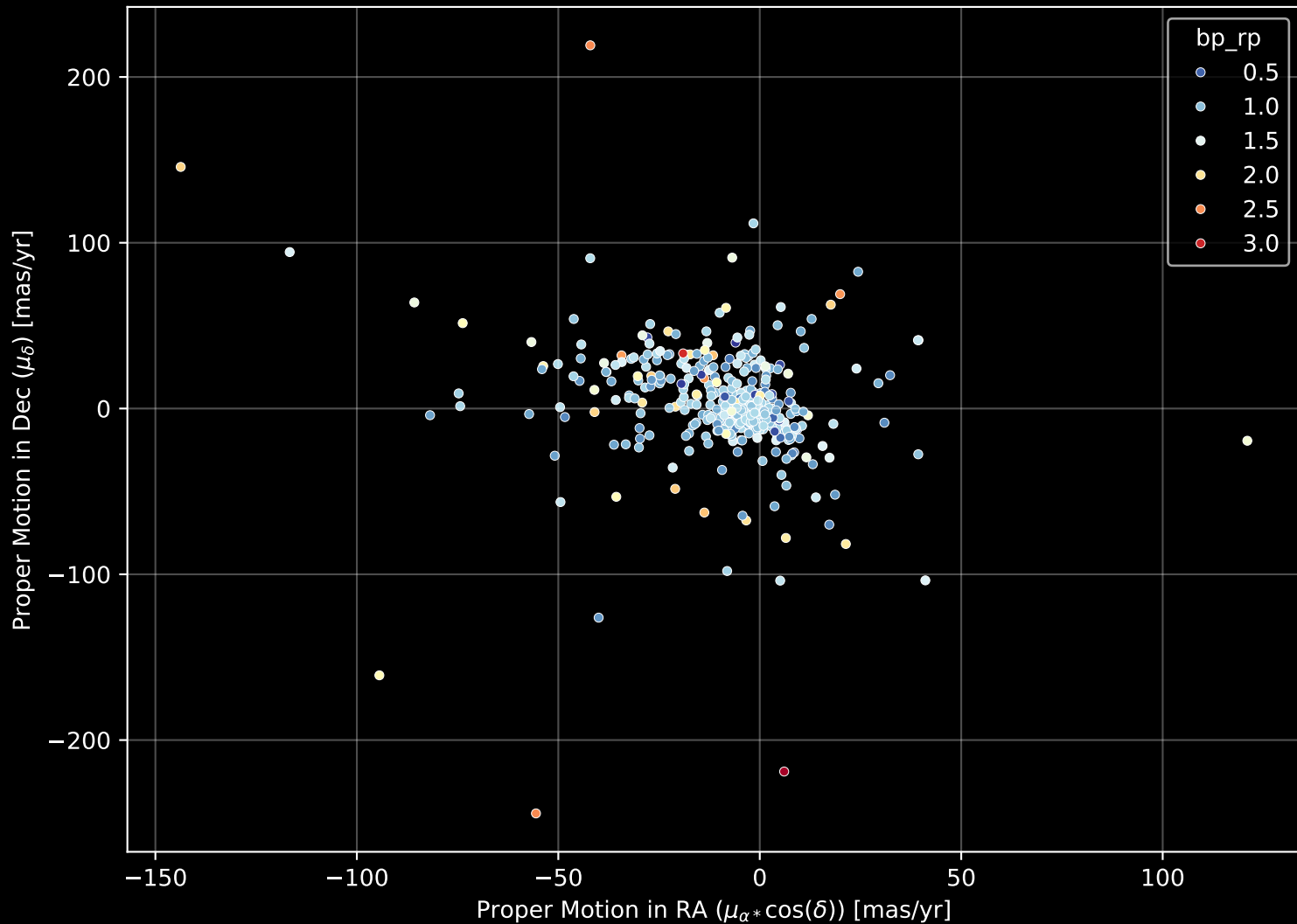
APOGEE DR17 Field: [N6229] Proper Motion Diagram (n= 485)
