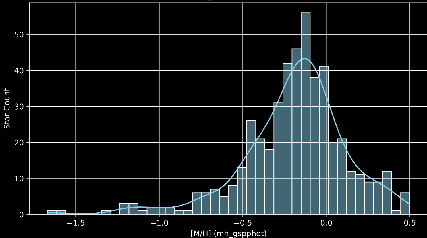
APOGEE DR17 Field: [N6229 [M/H] (mh_gspphot) (n= 483)
