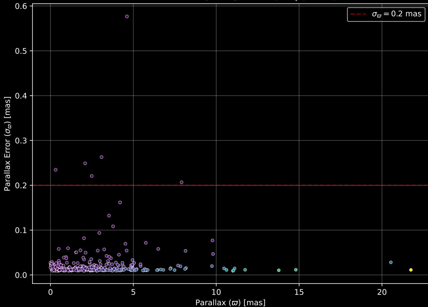
APOGEE DR17 Field: [N6229] Parallax Quality (n= 485)
