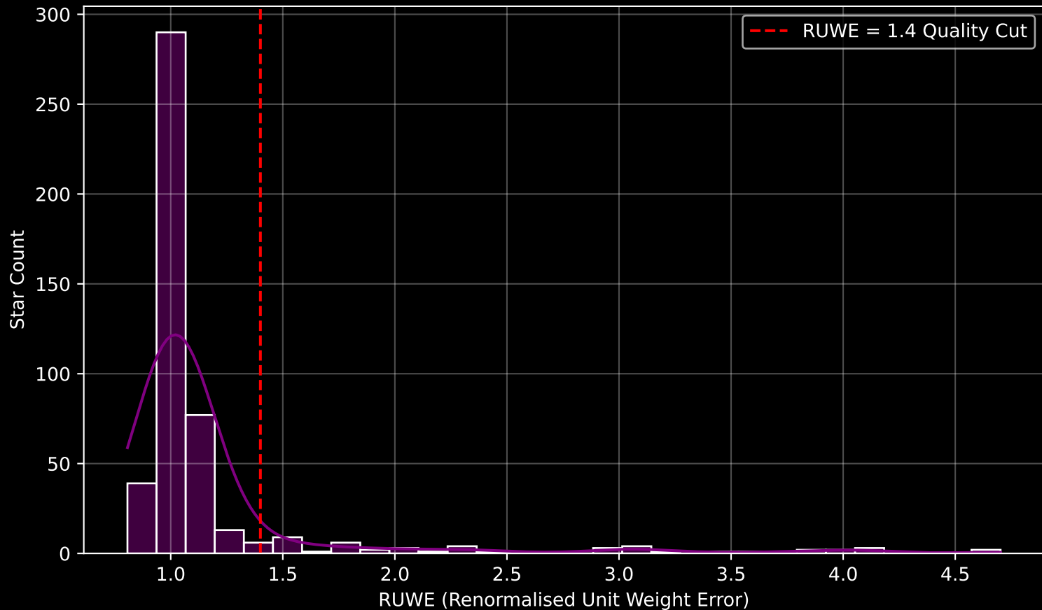
GAPOGEE DR17 Field [N6229] RUWE Distribution (n= 472)
