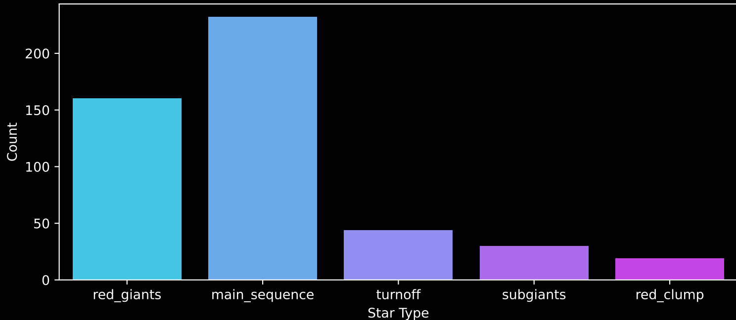
APOGEE DR17 Field: [N6229] Count plot of Star Type
