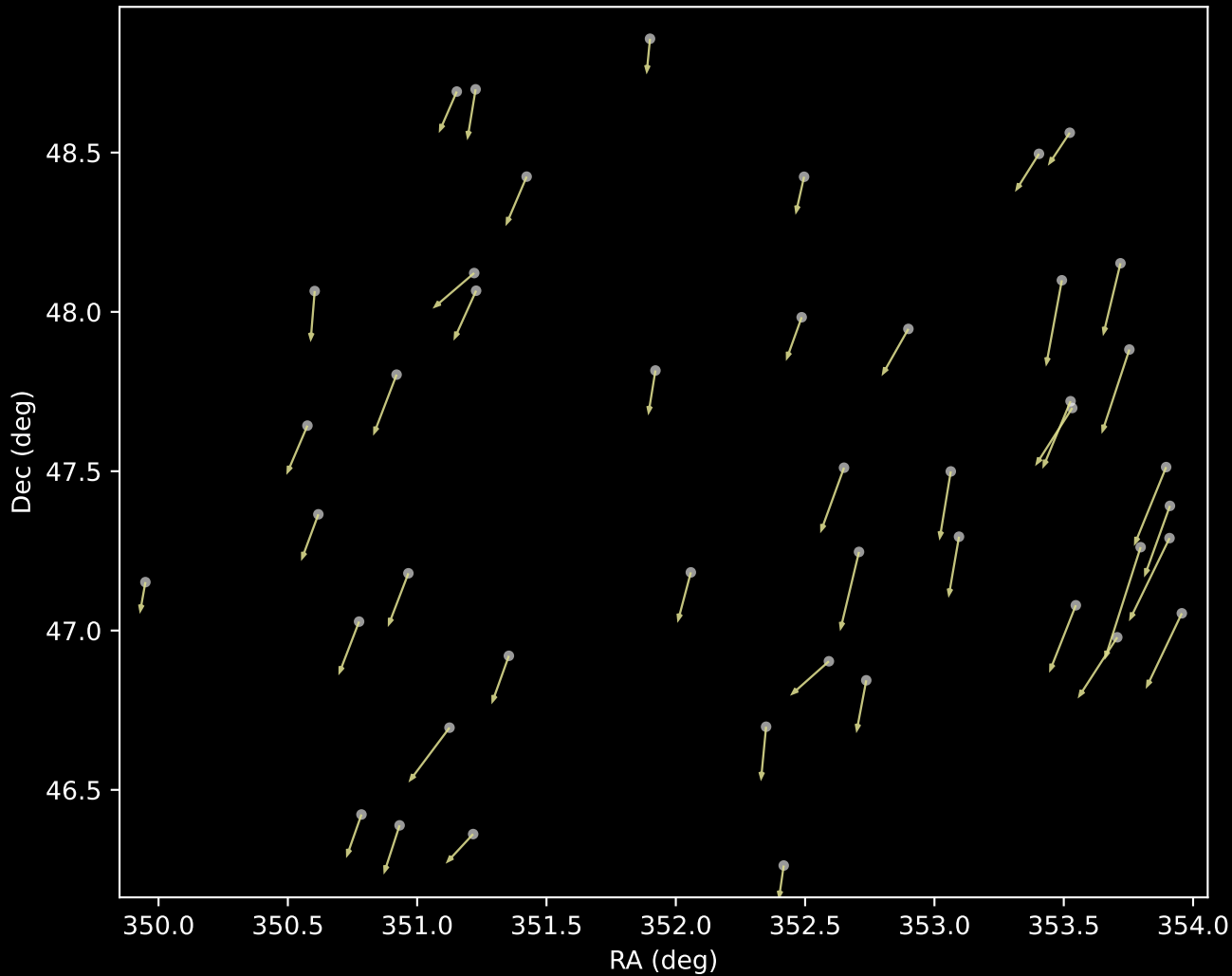
APOGEE DR17 Cluster 17 Proper Motion Vectors (n=45)
